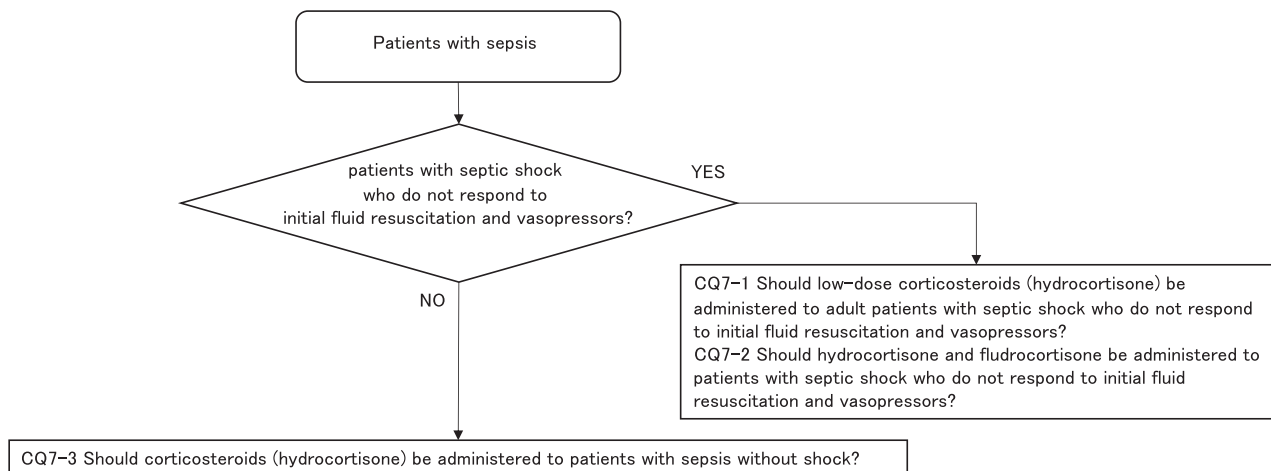
Fig. 6. CQ7: Corticosteroid therapy (clinical flow).
