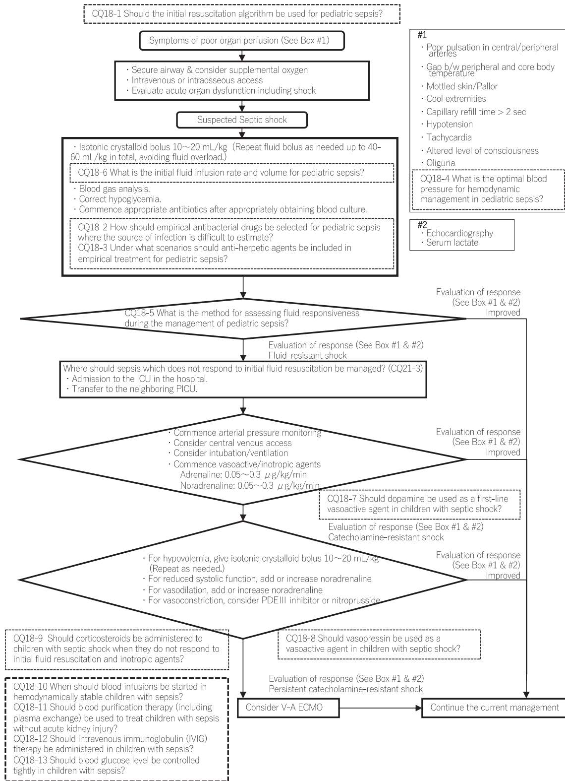
Fig. 17. CQ18: Management algorithm for pediatric septic shock (clinical flow).
