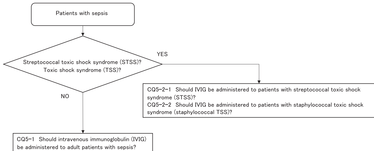
Fig. 4. CQ5: Intravenous immunoglobulin therapy (clinical flow).
